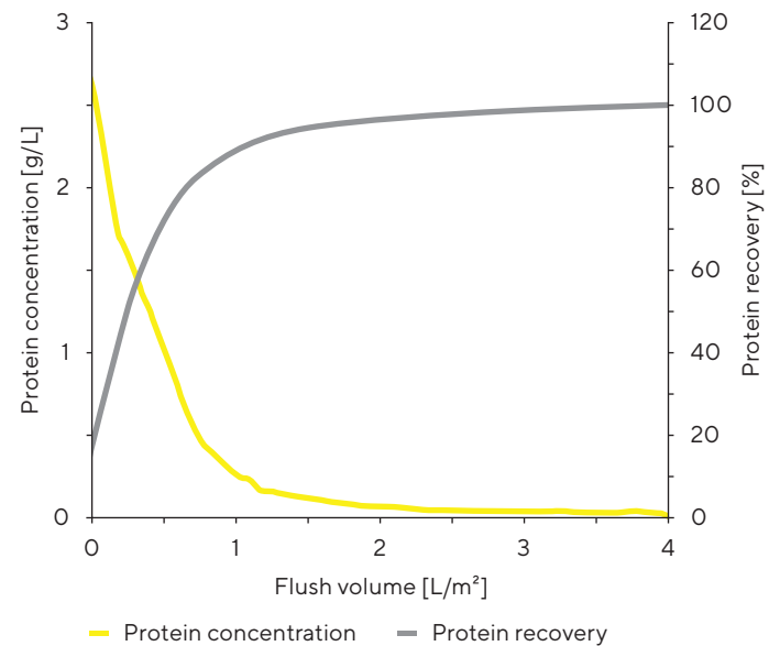
Figure 11: Post-flushing volume for Virosart® HF
