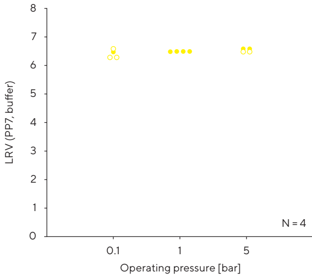
Figure 29: Different operating pressures of 0.1 bar, 1.0 bar and 5.0 bar tested on PP7 retention for Virosart® HF
