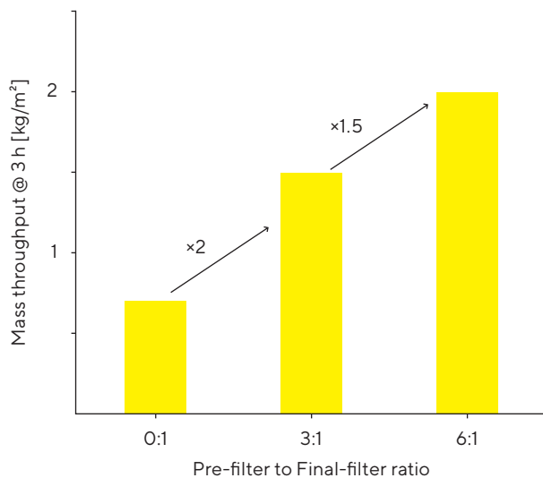
Figure 16: Optimization of adsorptive pre-filter area can improve overall virus-filter throughput
